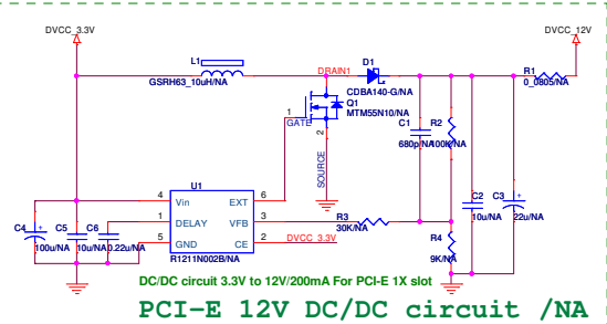
PCI-E 12V DC/DC circuit /NA
