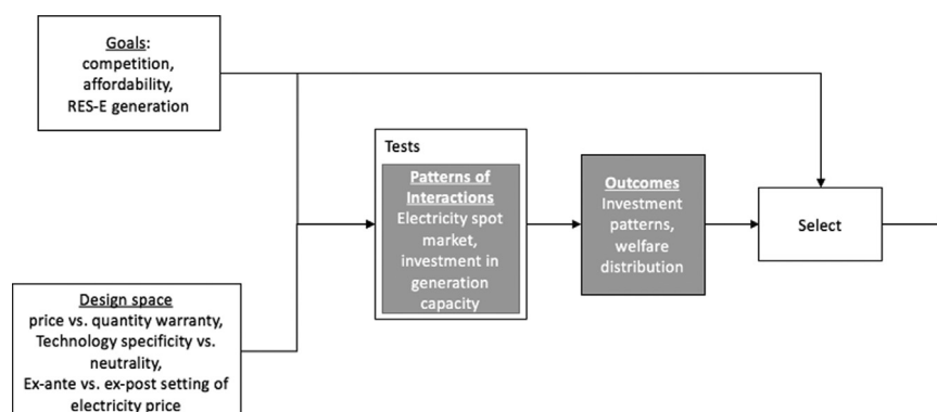
Fig. 6. Design space is evaluated by simulating patterns of interactions.
