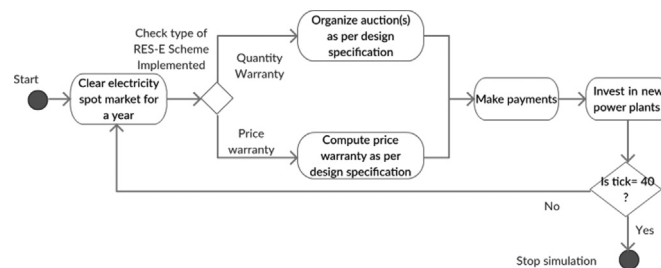
Fig. A2. Flowchart - Implementation of RES-E Policies.
