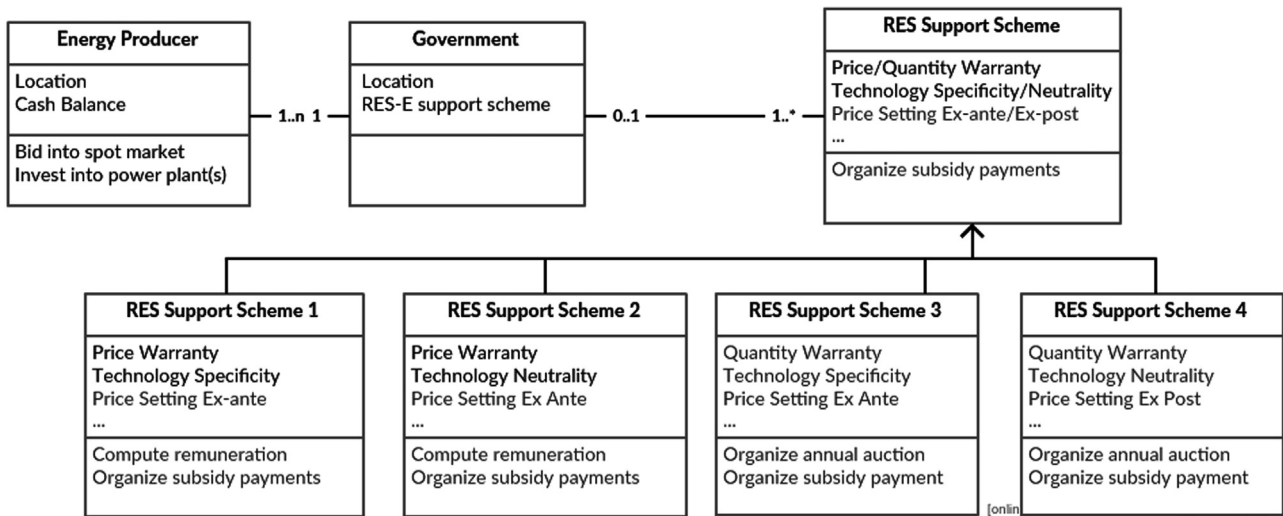
Fig. A1. Specification of class structure.
