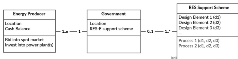
Fig. 7. Specification of class structure for generic design elements.
